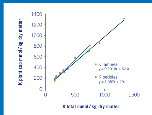
Figure 2: Correlation between K content in a tomato leaf determined by dry matter analysis and plant sap analysis. (Source: Cees Sonneveld and Wim Voogt 2009)
